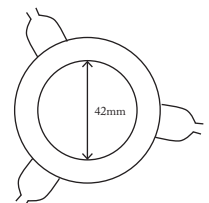
ES Edison Screw 42mm internal diameter.
